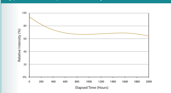
Typical Lamp Intensity Over Lifetime
